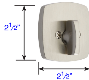
Interior Trim (8426) • Projection is \frac{1}{16} " • Thickness is \frac{3}{8} "
