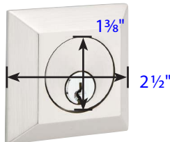
Exterior Trim (8478) • Projection is \frac{1}{2} " • 8378 same on both sides
